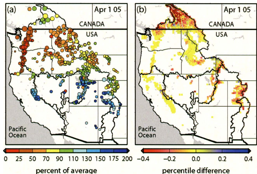
Fig. 3. Snow assimilation is effected by merging, at forecast initiation time, (a) the measured SWE anomalies at NRCS SNOTEL and Environment Canada snow pillow stations with the modeled SWE anomalies, resulting in (b) varying adjustments to the model-only snow-water equivalent, as reflected by the change in SWE percentile.
