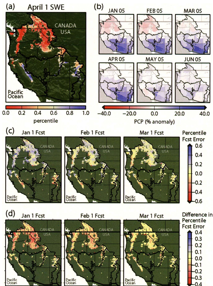
FIG. 6. (a) 1 Apr 2005 SWE percentile from real-time nowcast; (b) CPC precipitation forecast (16 Dec) used in 1 Jan 2005 hydrologic forecast; (c) percentile error in CPC-based mean forecast of 1 Apr 2005 SWE percentile for leads of 1–3 months; and (d) difference in CPC-based forecast percentile absolute error from ESP-based forecast percentile absolute error (negative for lower CPC errors).
